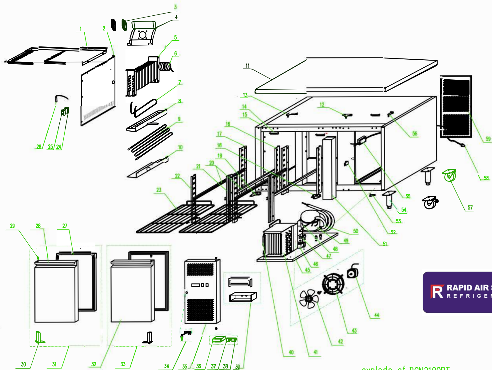
explode of RGN2100BT
